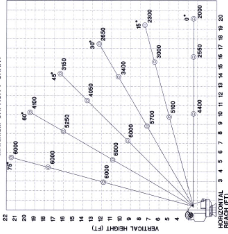
HT40KX - 10-16-20 BOOM MAXIMUM CAPACITY CHART
